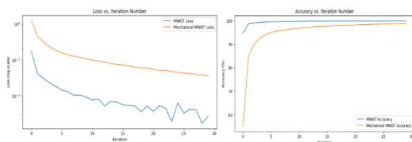
Figure 6: CNN loss and accuracy curves vs. epochs on mechanical MNIST, illustrating robust convergence.
