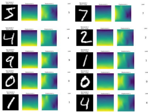
Figure 5: Visuals of mechanical MNIST training and test performance.
