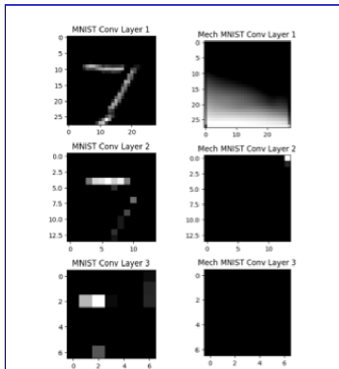
Figure 3: Feature maps for digit 7 across three convolutional layers, comparing MNIST and mechanical MNIST shear effects.
