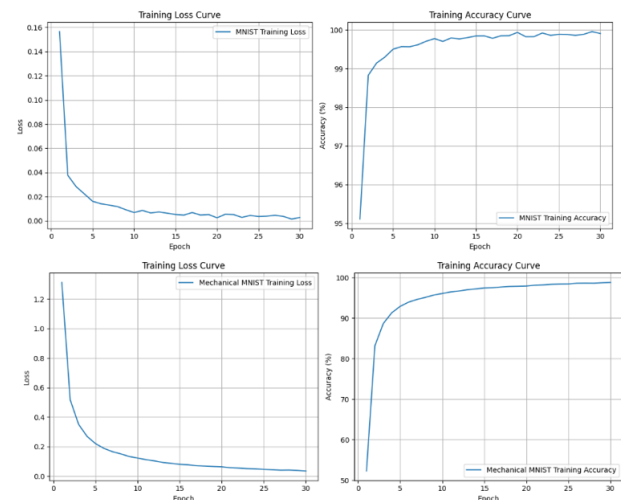
Figure 4: Training loss and accuracy for CNN on Mechanical MNIST, demonstrating rapid convergence under shear perturbations.
